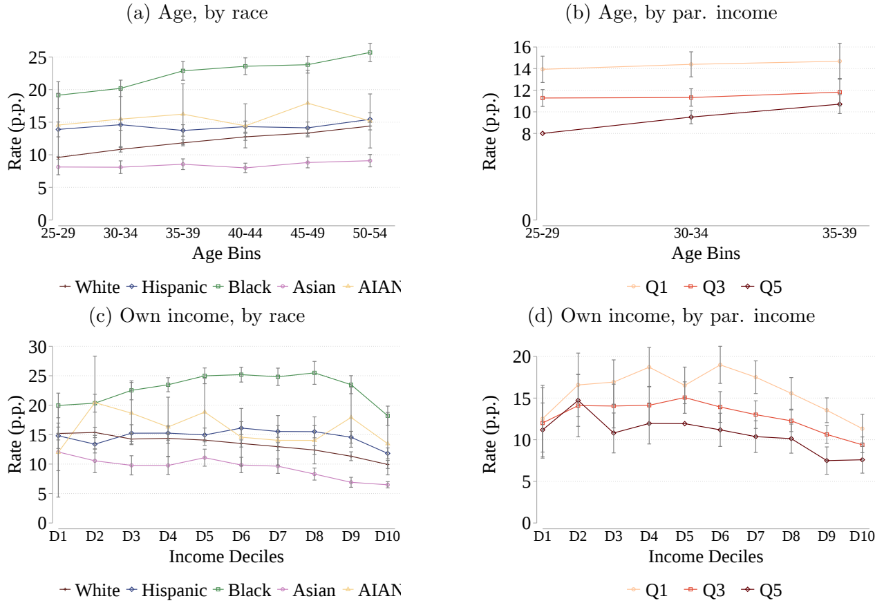
Figure A.10: Withdrawal probabilities across different specifications
